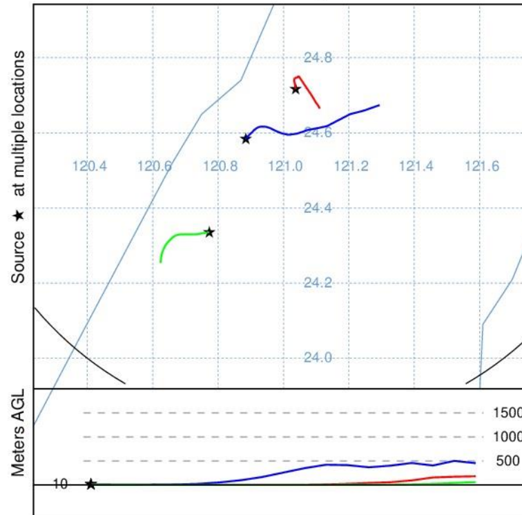
Forward trajectories starting at 2000 UTC 18 Mar 20 AWRF Meteorological Data
