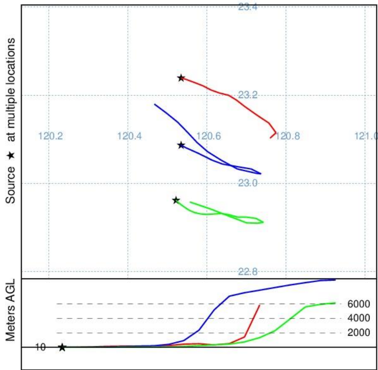
Forward trajectories starting at 0400 UTC 18 Aug 20 AWRF Meteorological Data
