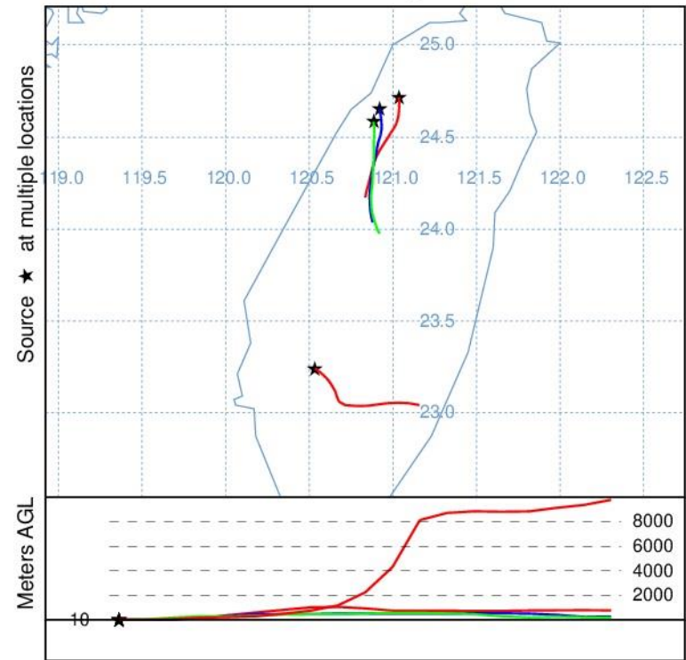
Forward trajectories starting at 0600 UTC 03 Sep 20 AWRF Meteorological Data
