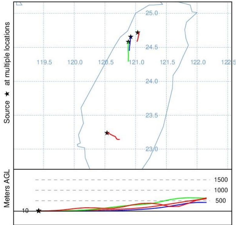
Forward trajectories starting at 0100 UTC 03 Sep 20 AWRF Meteorological Data
