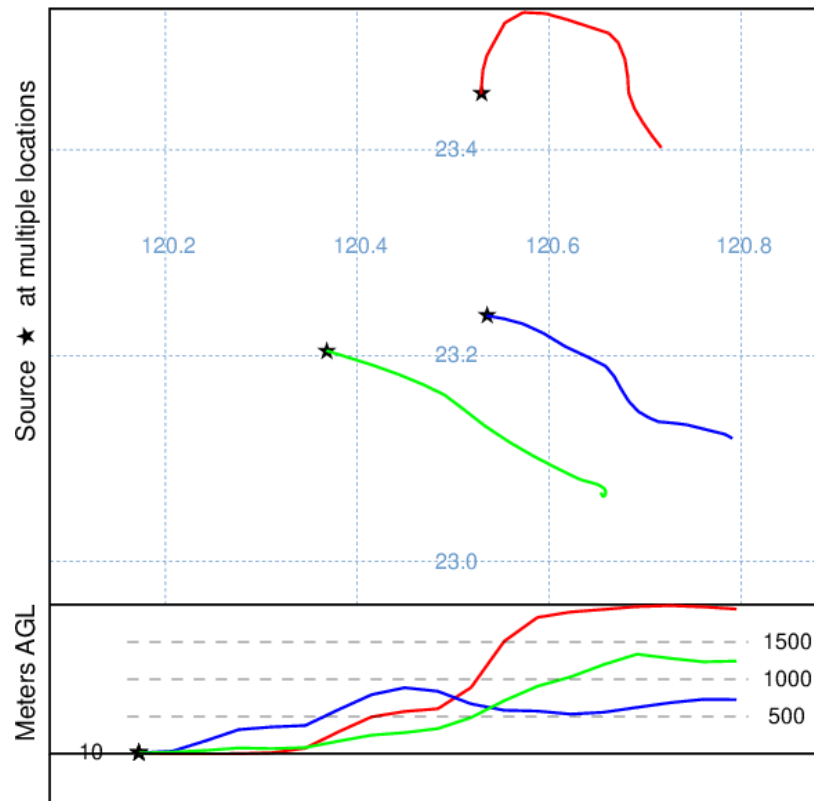
Forward trajectories starting at 0600 UTC 10 Sep 20 AWRF Meteorological Data
