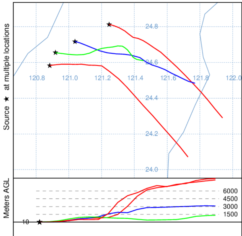
Forward trajectories starting at 0500 UTC 10 Sep 20 AWRF Meteorological Data
