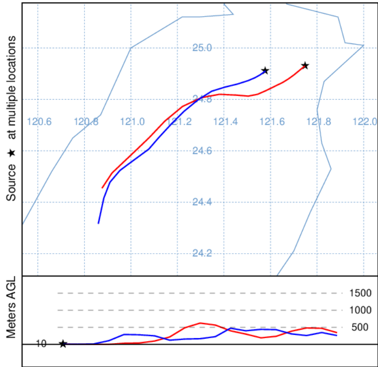
Forward trajectories starting at 0400 UTC 29 Oct 20 AWRF Meteorological Data
