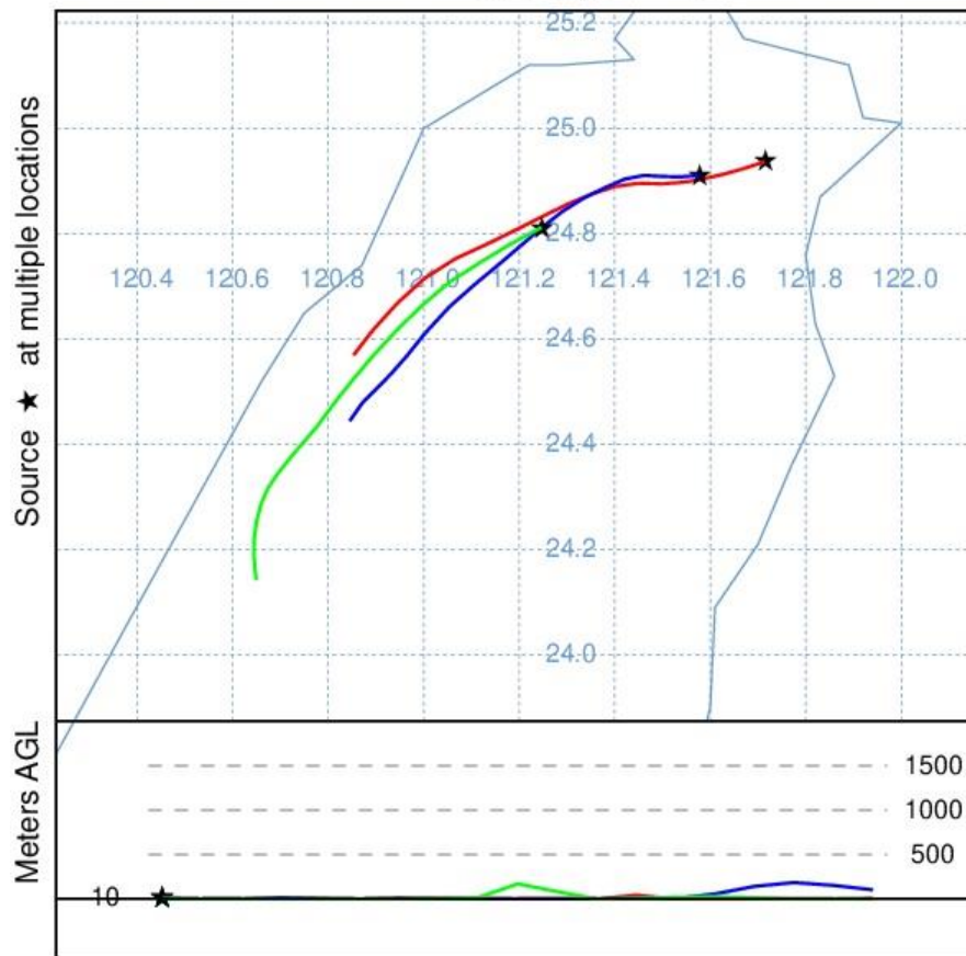
Forward trajectories starting at 0600 UTC 12 Nov 20 AWRF Meteorological Data
