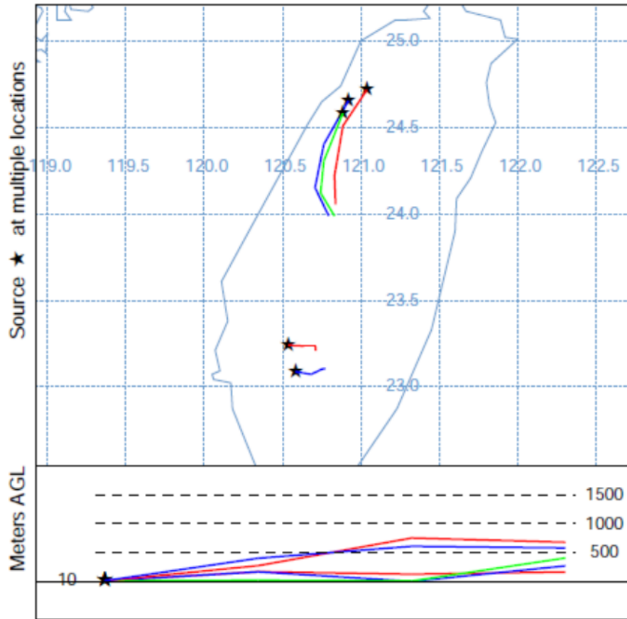
Forward trajectories starting at 0300 UTC 17 Jan 22 AWRF Meteorological Data
