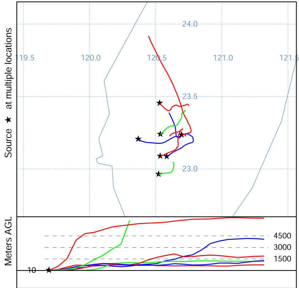
Forward trajectories starting at 0600 UTC 26 Jun 23 AWRF Meteorological Data
